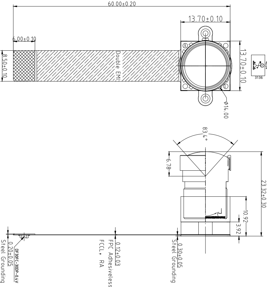
TOP VIEW
