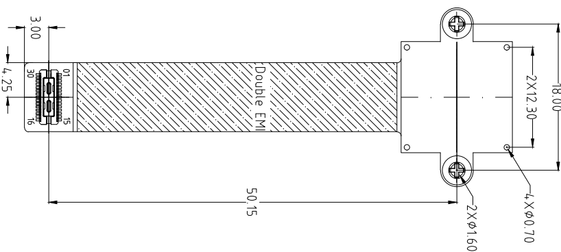
BOTTOM VIEW
